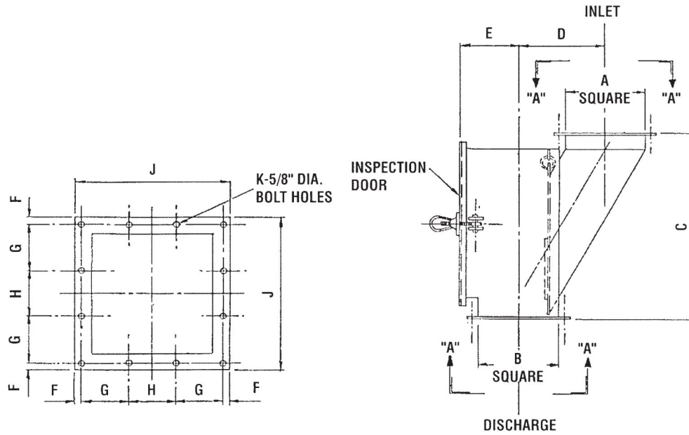
VIEW "A-A" (INLET AND DISCHARGE FLANGE)
